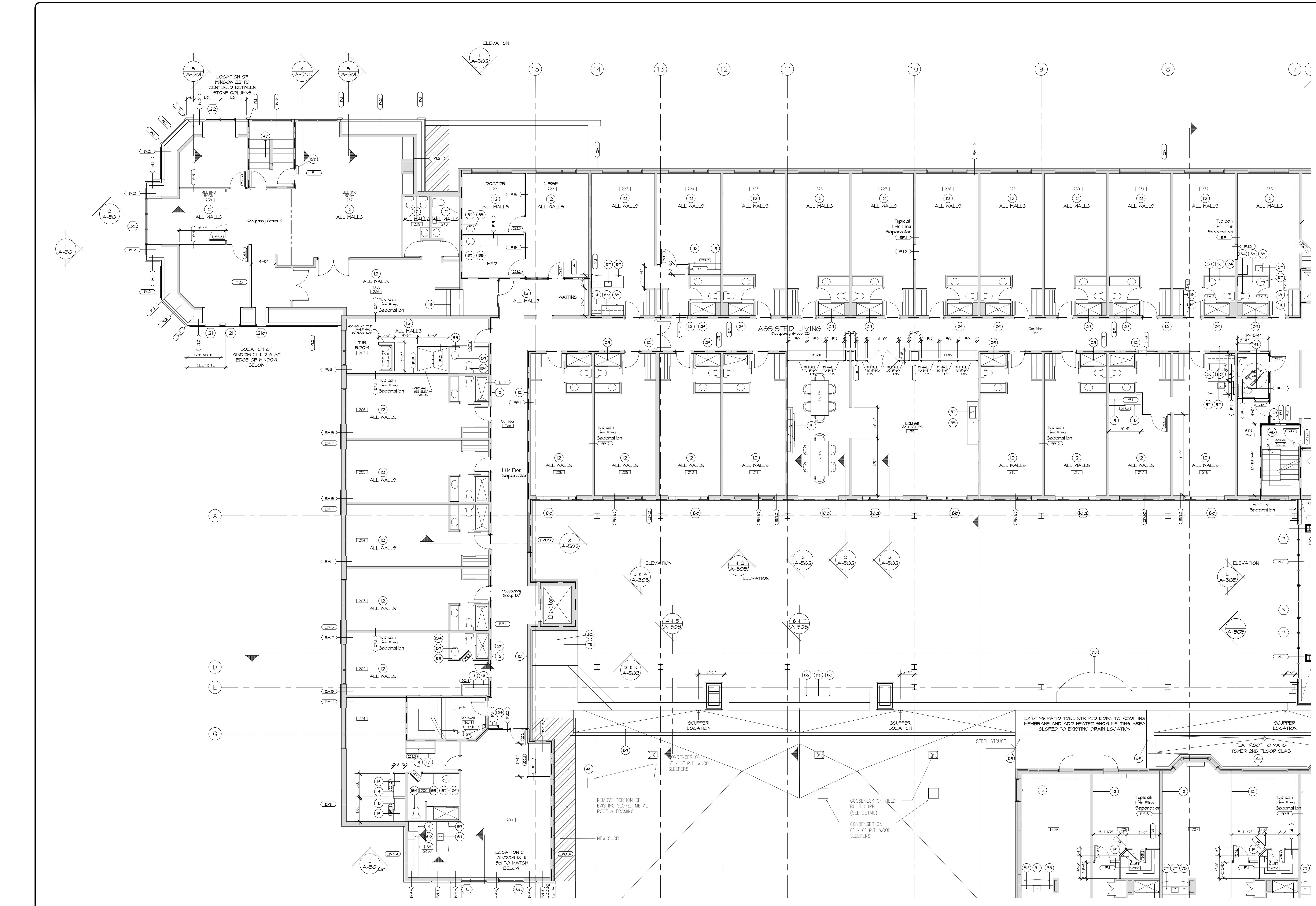
1 SECOND FLOOR - ATRIUM/SOLARIUM & ASSISTED LIVING WING SCALE: 1/8" = 1'-0"
