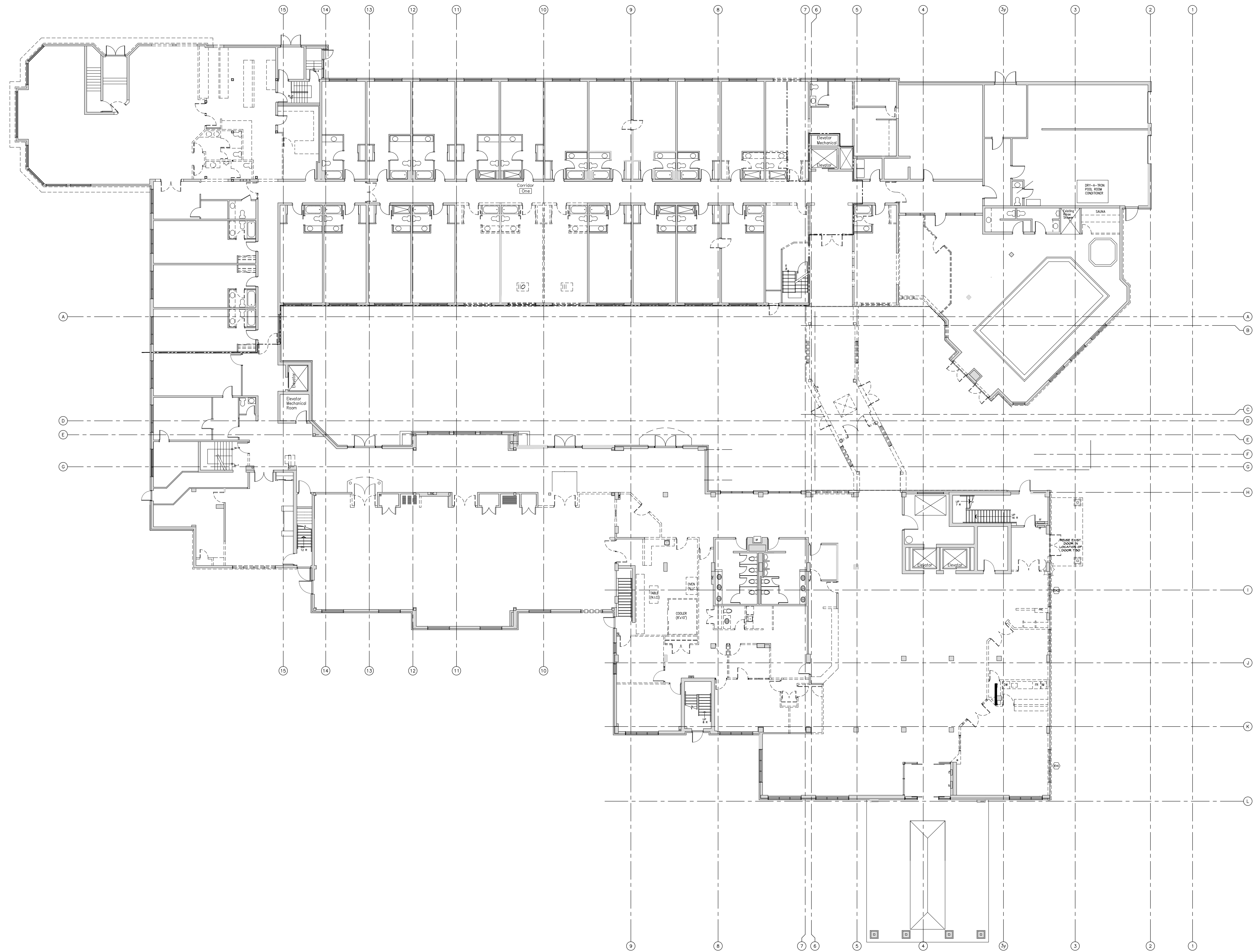
DEMOLITION EXISTING GROUND FLOOR SCALE: 1/16" = 1'-0"
