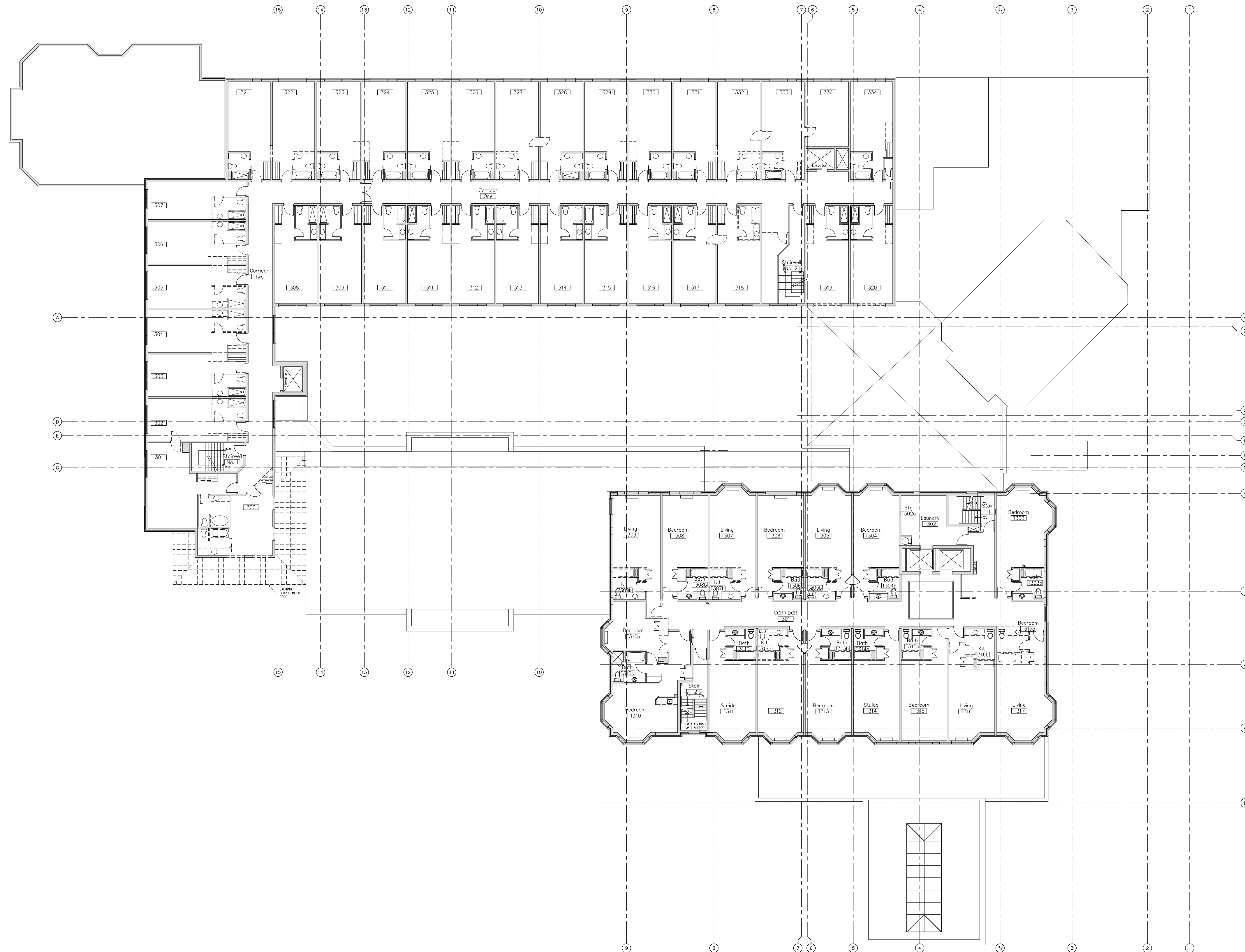
DEMOLITION EXISTING THIRD FLOOR A-303 / SCALE: 1/16" = 1'-0"
