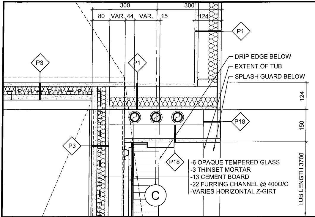
20 503 TYPICAL WATER FEATURE DETAIL SCALE = 1:10
