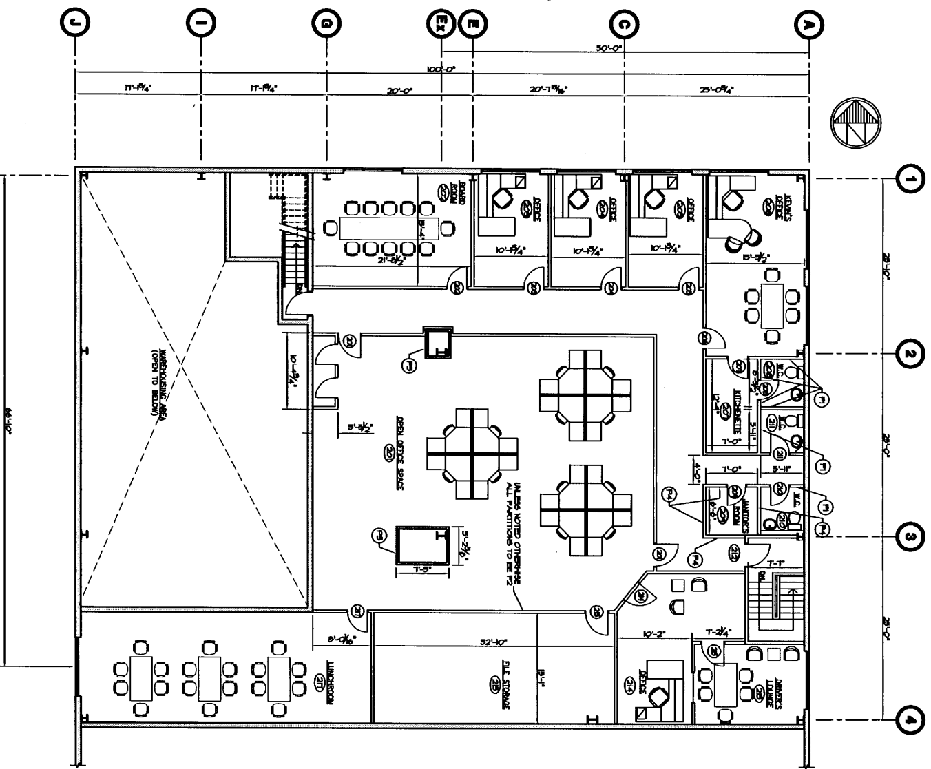
SECOND FLOOR OFFICE LAYOUT PLAN 1/8" = 1'-0"
