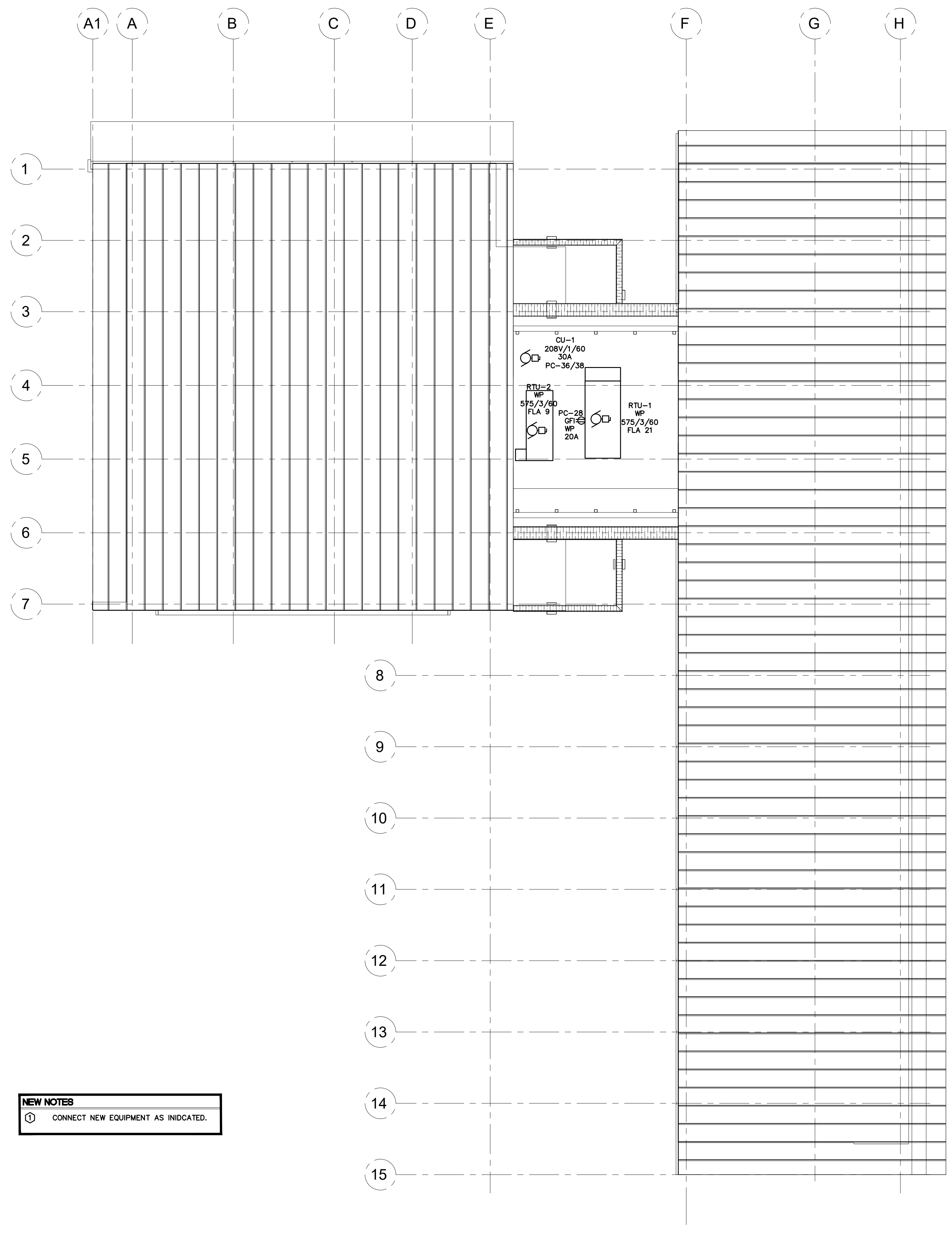
2 ROOF PLAN E202 SCALE: 1:100
