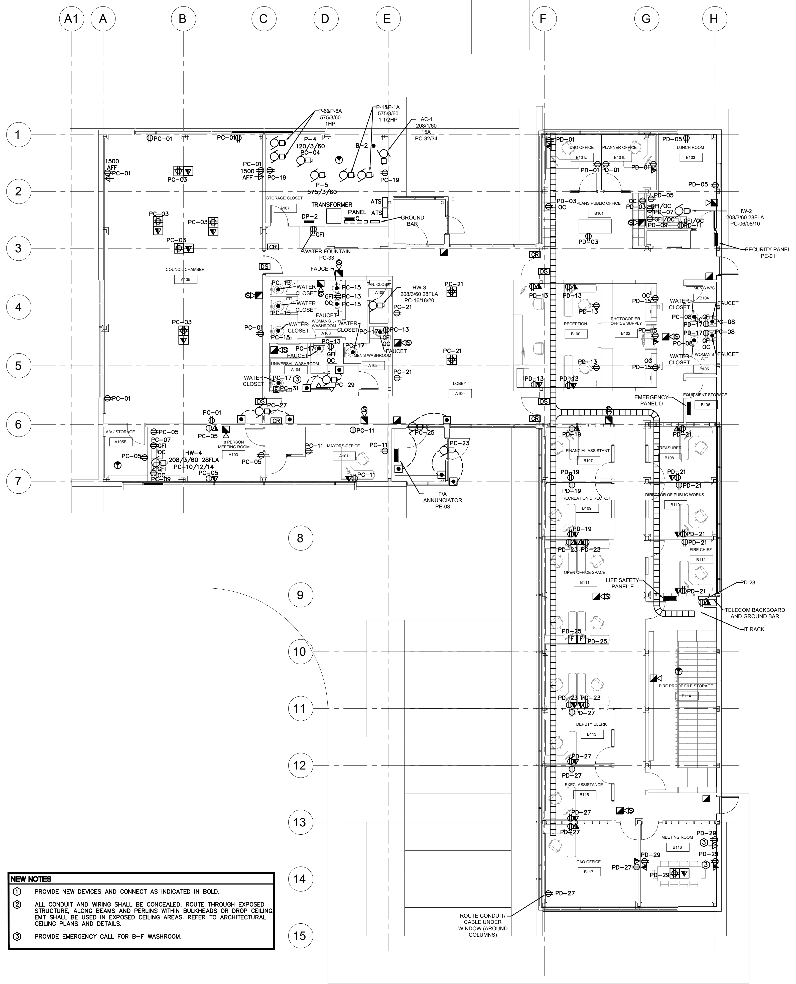
1 FLOOR PLAN E202 SCALE: 1:100
