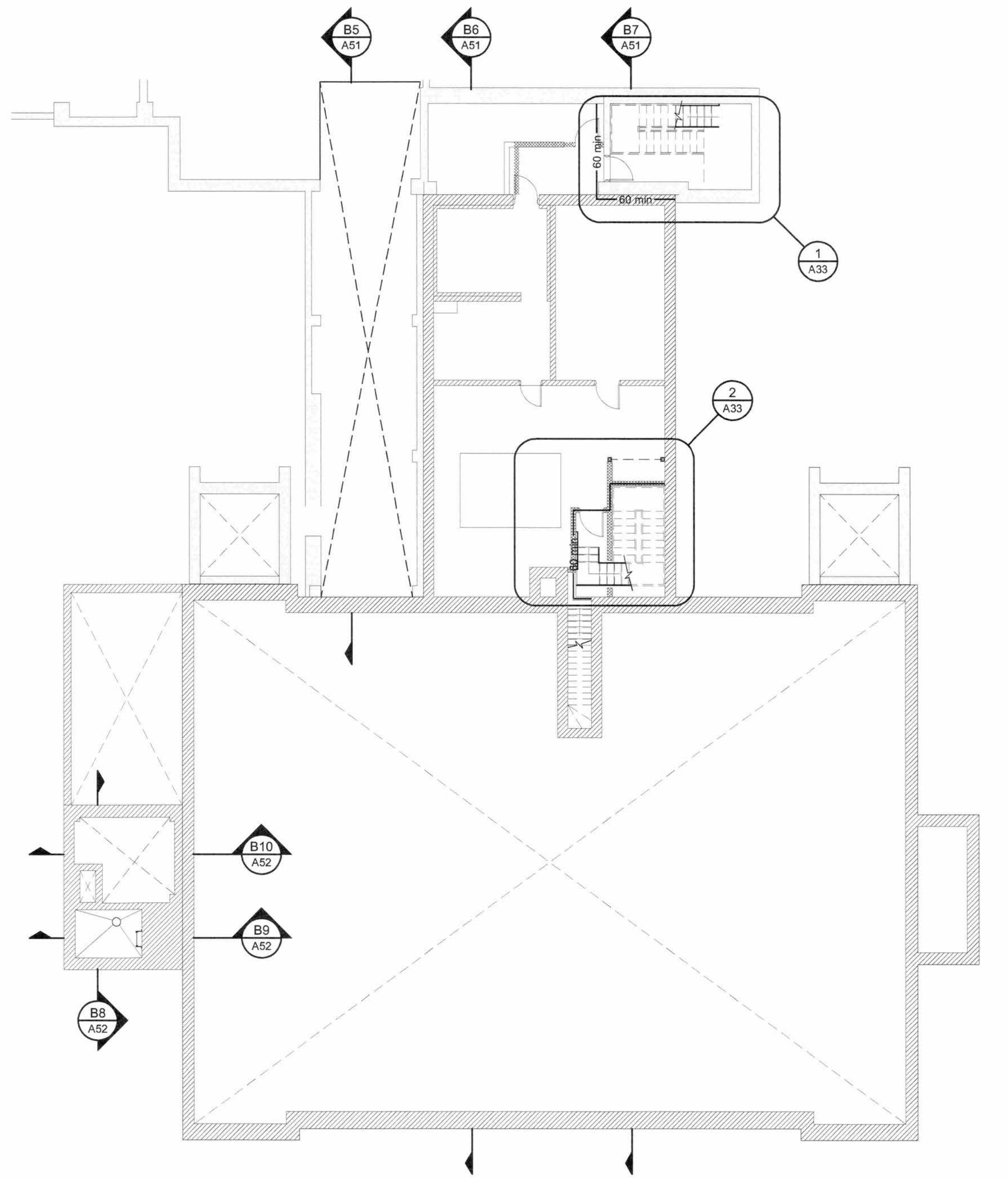
1 BASEMENT FIRE SEPARATION PLAN SCALE: 3/32" = 1'-0"
