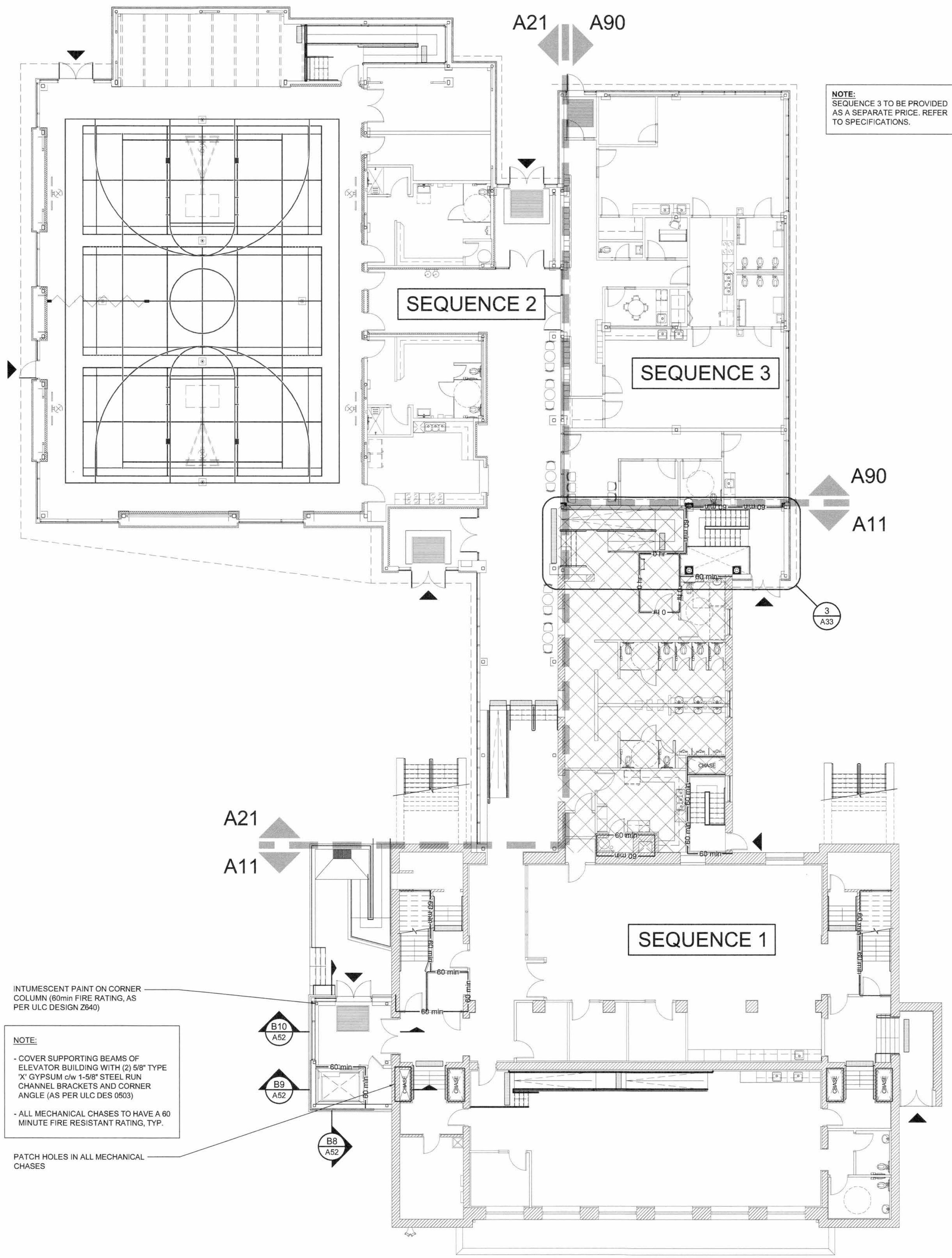
2 GROUND FIRE SEPARATION PLAN SCALE: 3/32" = 1'-0"
