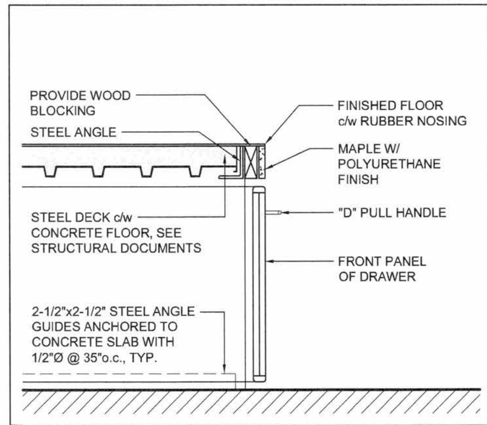
4 STAGE NOSING DETAIL SCALE: 1" = 1'-0"
