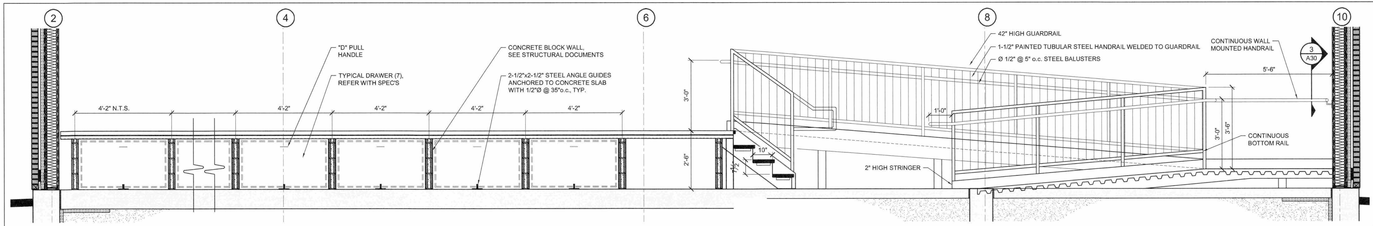
2 STAGE AND RAMP SECTION SCALE: 1/2" = 1'-0"
