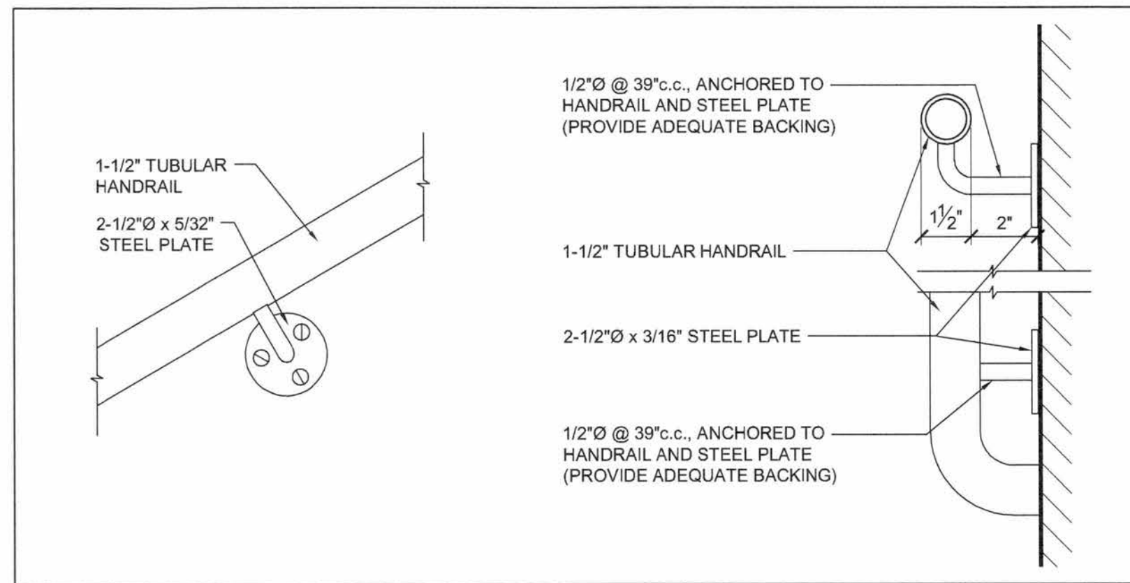
3 HANDRAIL SECTION DETAIL SCALE: 3" = 1'-0"
