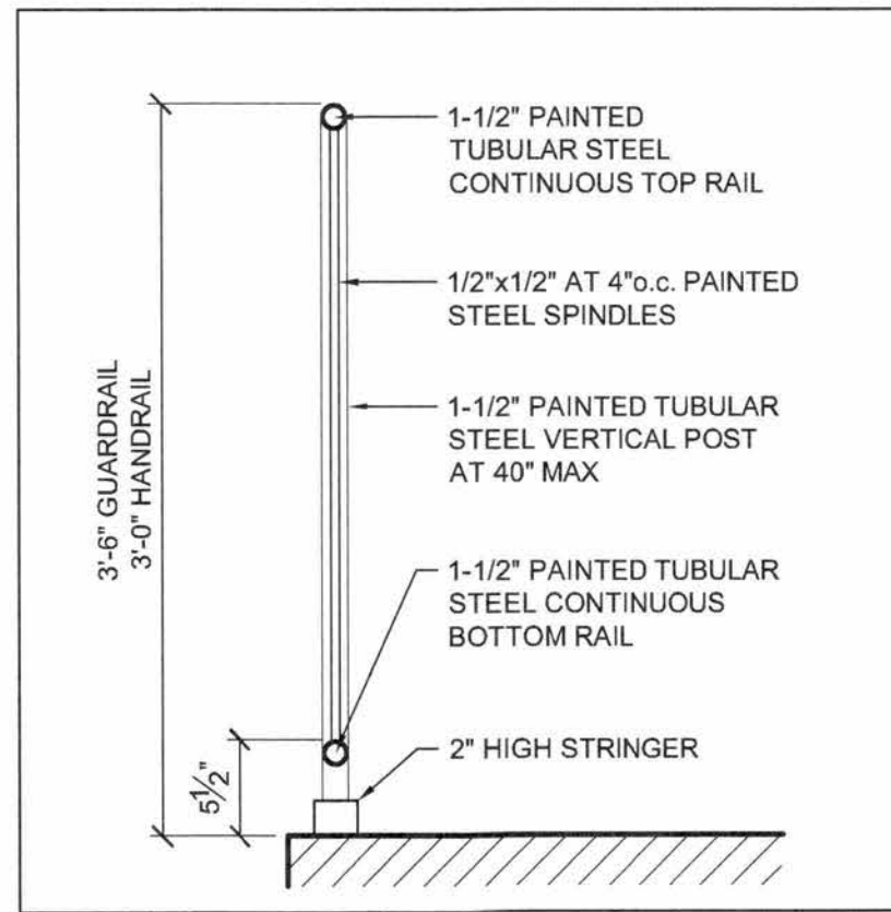
5 HANDRAIL OR GUADRAIL DETAIL SCALE: 1" = 1'-0"
