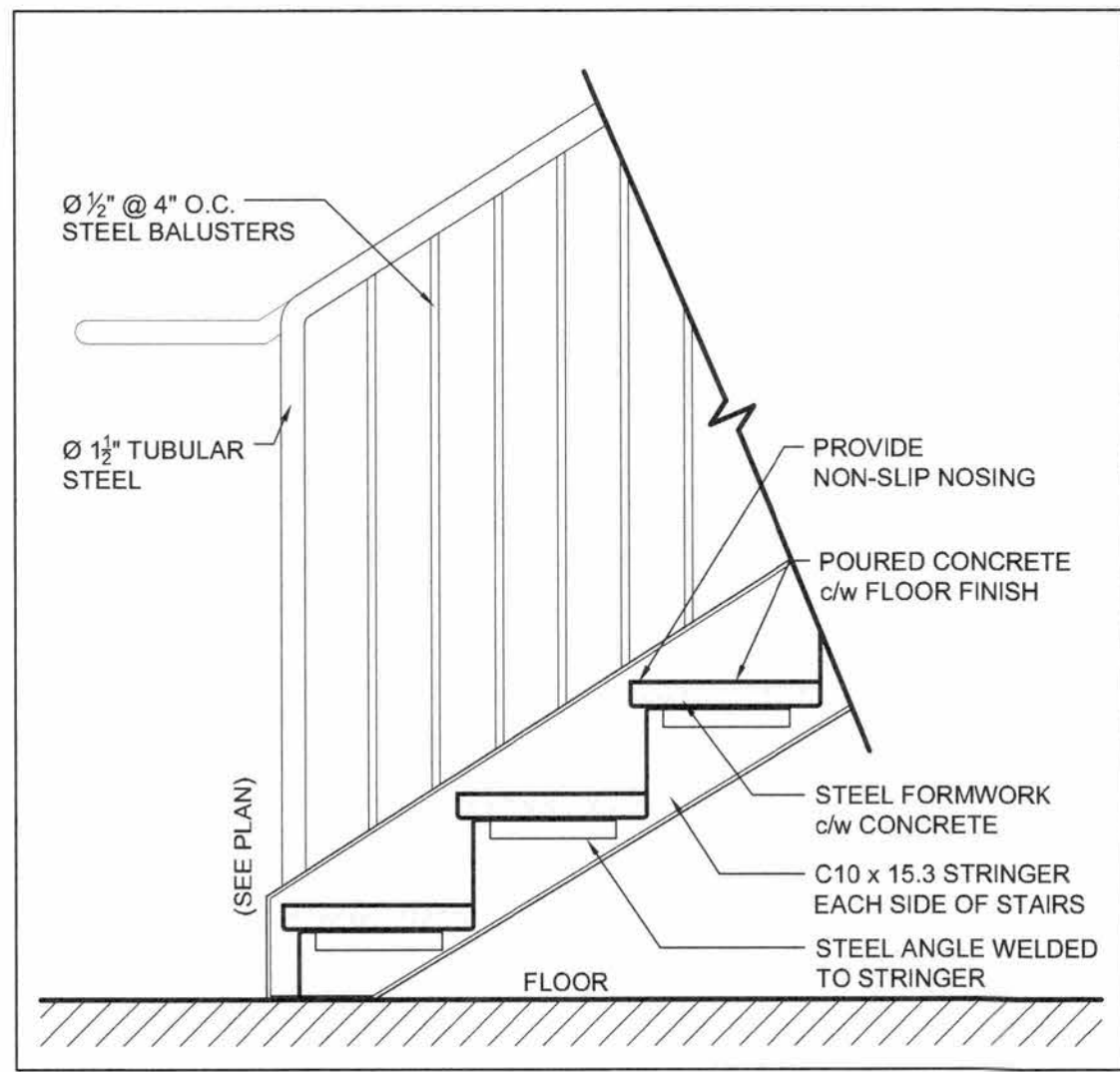
6 TYPICAL STAIR DETAIL SCALE: 1" = 1'-0"
