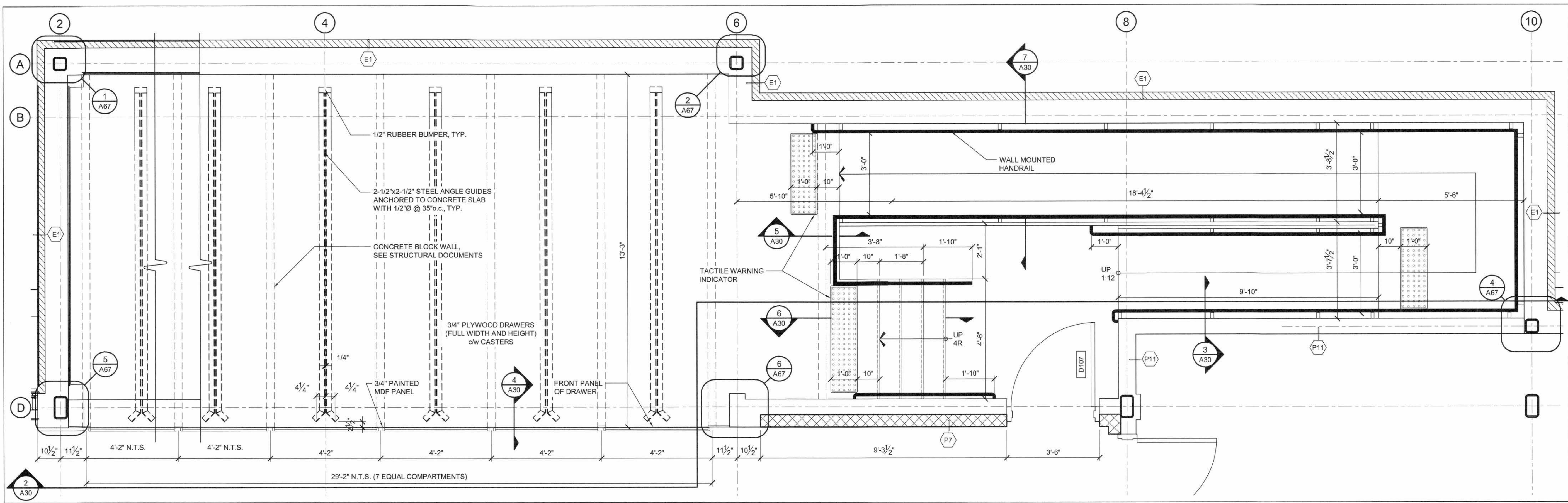
1 ENLARGED STAGE AND RAMP PLAN SCALE: 1/4" = 1'-0"
