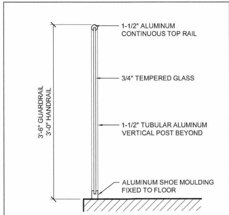
3 HANDRAIL OR GUARDRAIL DETAIL SCALE: 1" = 1'-0"
