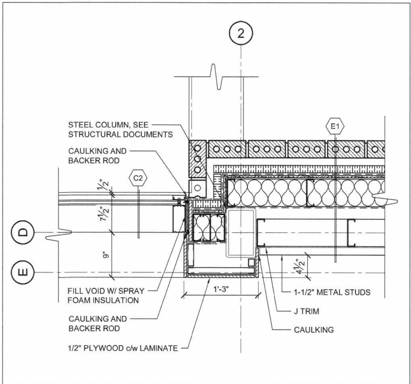
9 UPPER DETAIL @ GRIDLINE 2 AND D A67 SCALE: 1" = 1'-0"
