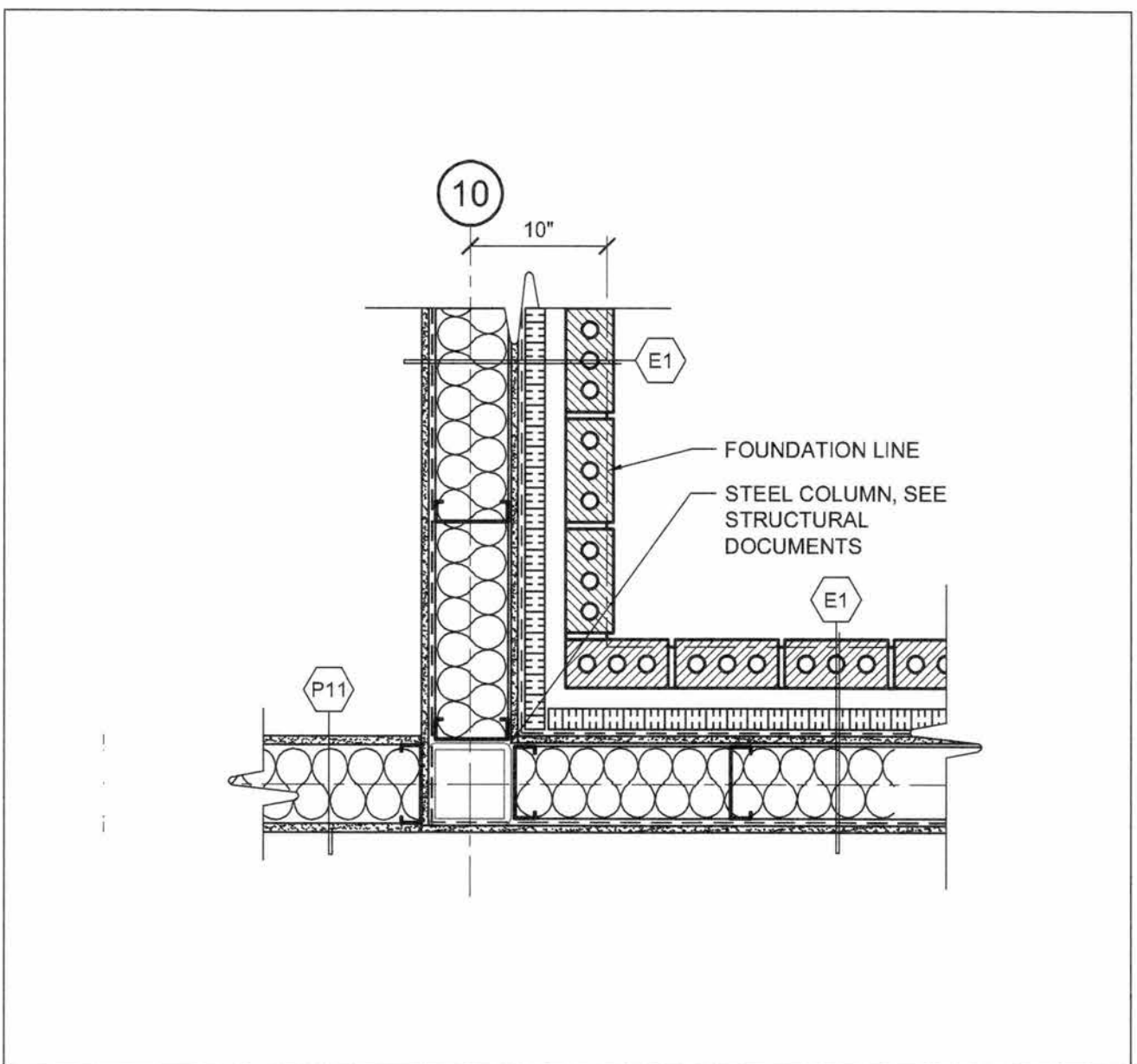
4 INTERIOR CORNER DETAIL A67 SCALE: 1" = 1'-0"
