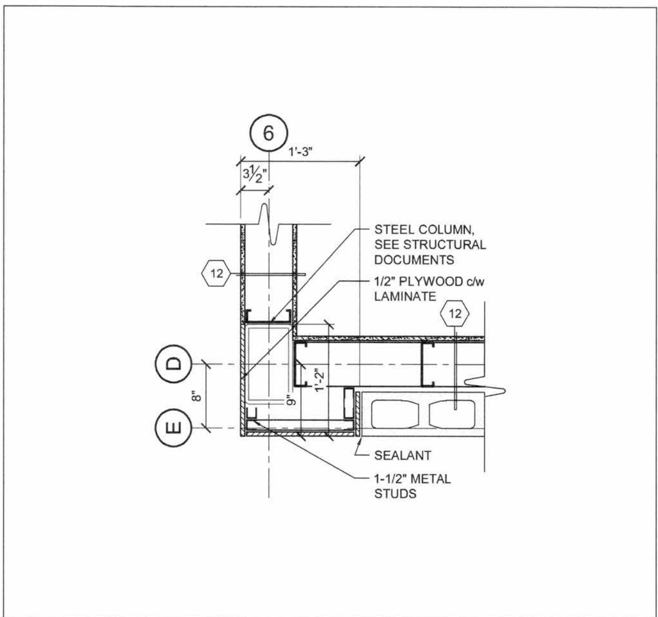
6 LOWER DETAIL @ GRIDLINE 6 AND D A67 SCALE: 1" = 1'-0"
