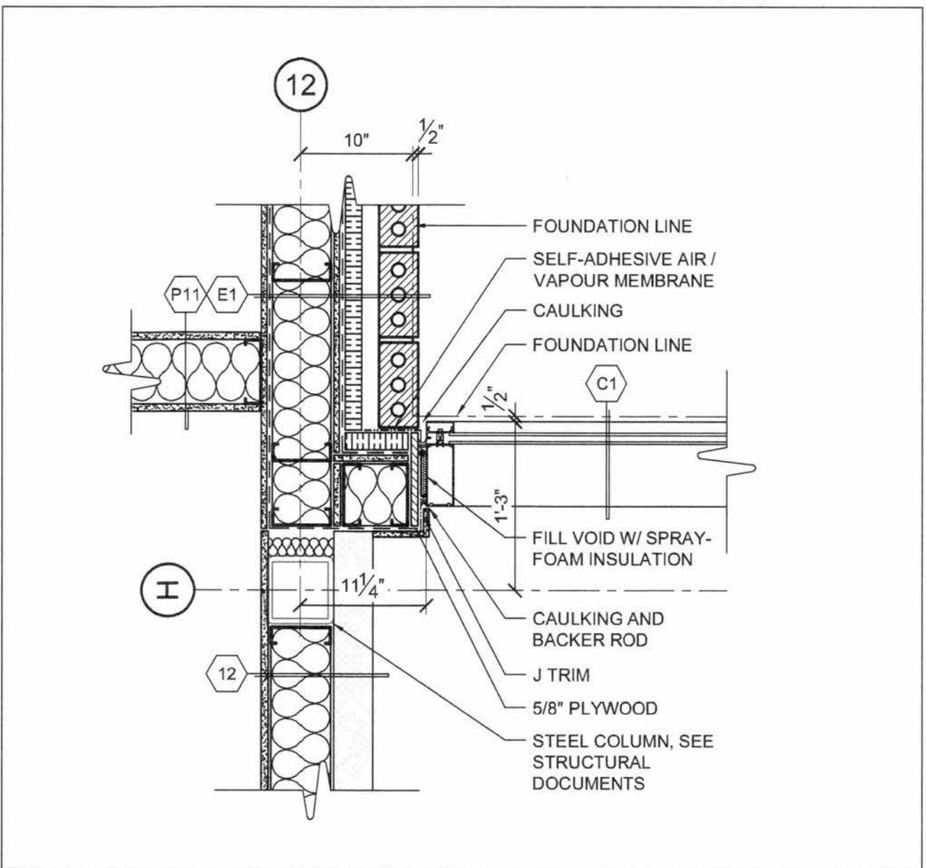
3 WINDOW JAMB DETAIL A67 SCALE: 1" = 1'-0"
