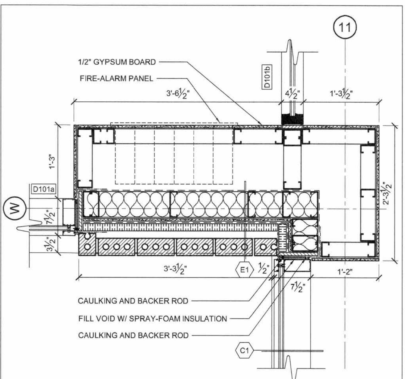
12 WINDOW JAMB DETAIL #2 A67 SCALE: 1" = 1'-0"
