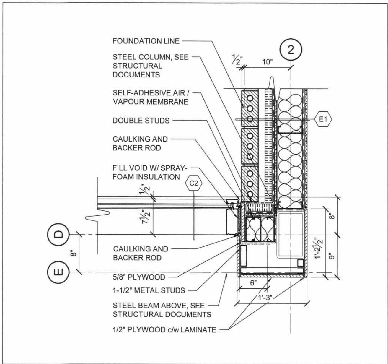
5 LOWER DETAIL @ GRIDLINE 2 AND D A67 SCALE: 1" = 1'-0"
