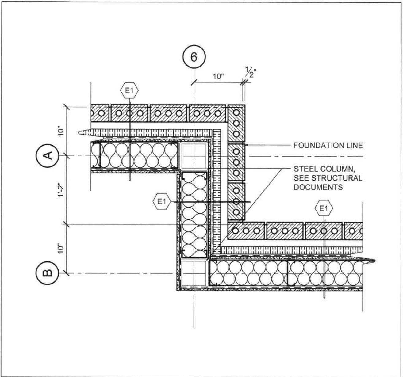
2 EXTERIOR AND INTERIOR CORNER DETAIL A67 SCALE: 1" = 1'-0"
