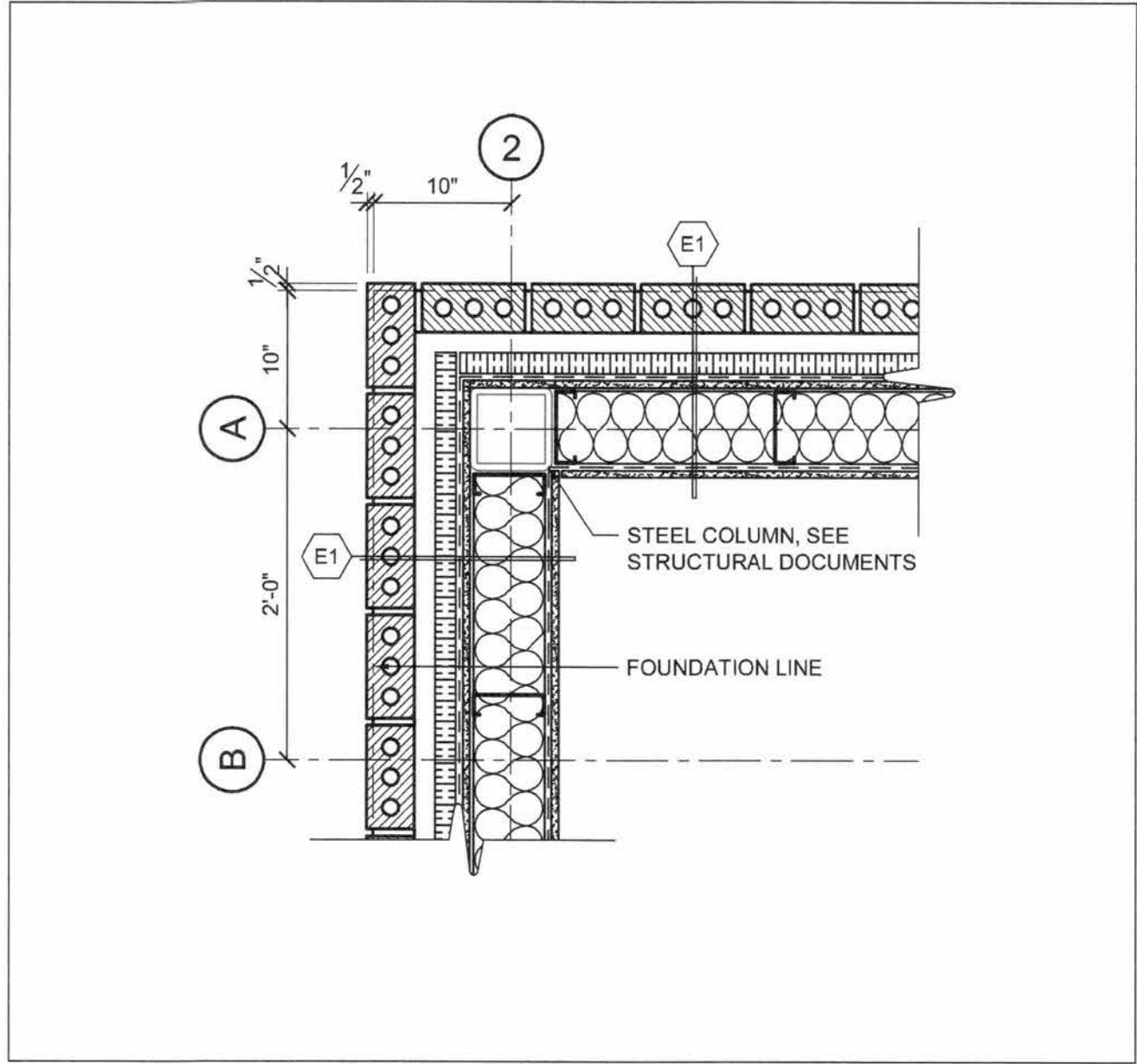
1 EXTERIOR CORNER DETAIL A67 SCALE: 1" = 1'-0"
