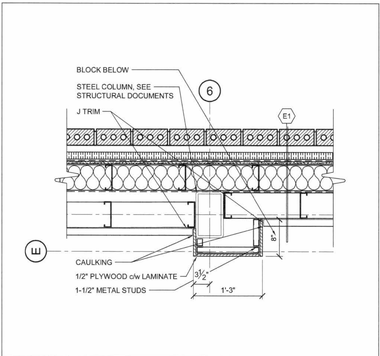
10 UPPER DETAIL @ GRIDLINE 6 AND E A67 SCALE: 1" = 1'-0"
