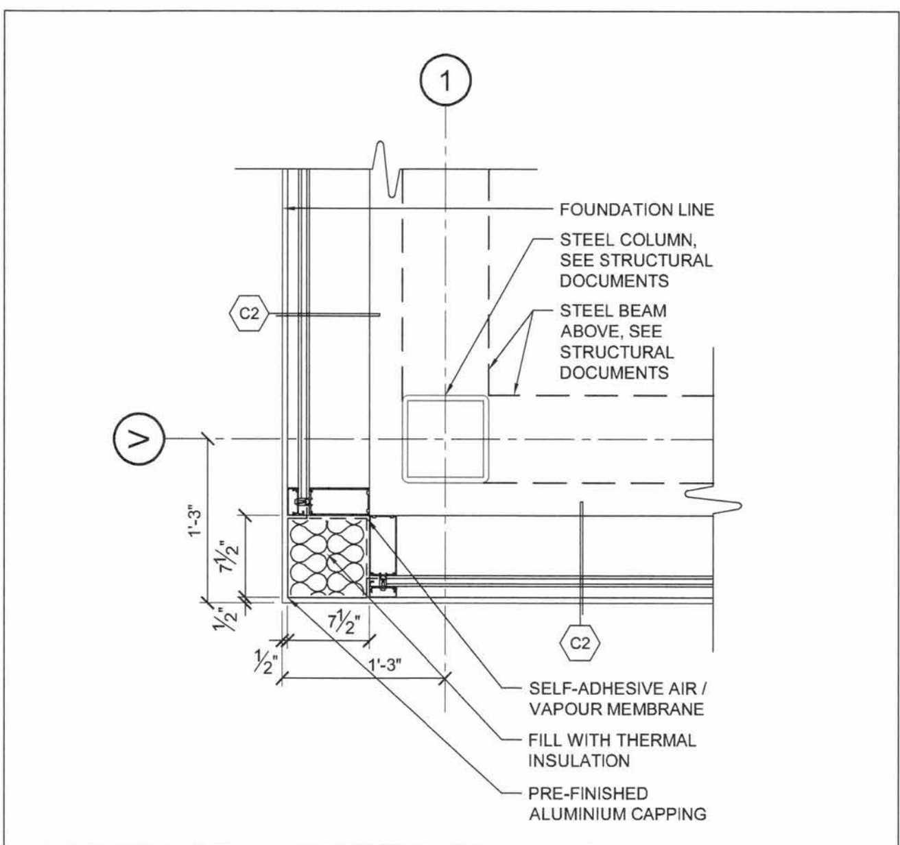
7 CURTAIN WALL @ CORNER DETAIL A67 SCALE: 1" = 1'-0"
