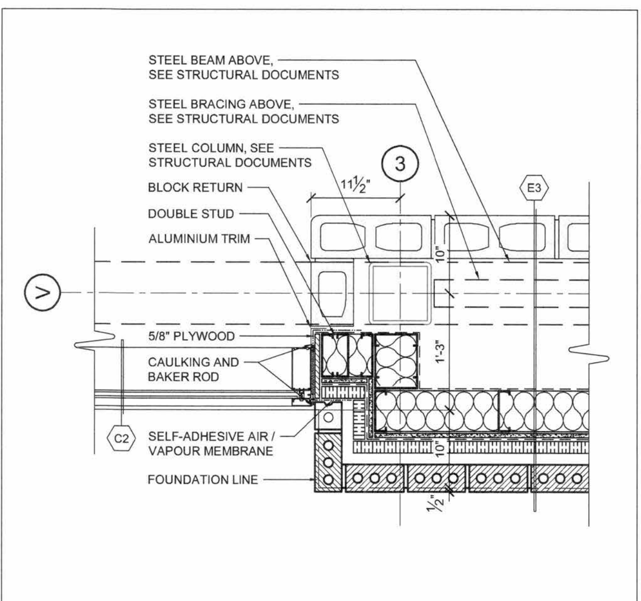
8 BRICK BUMP-OUT DETAIL A67 SCALE: 1" = 1'-0"
