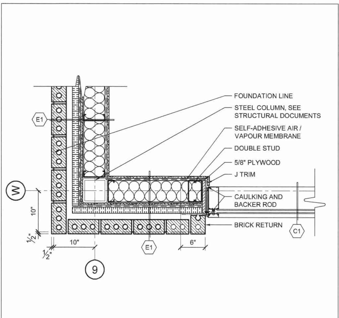
11 EXTERIOR CORNER AND WINDOW DETAIL A67 SCALE: 1" = 1'-0"
