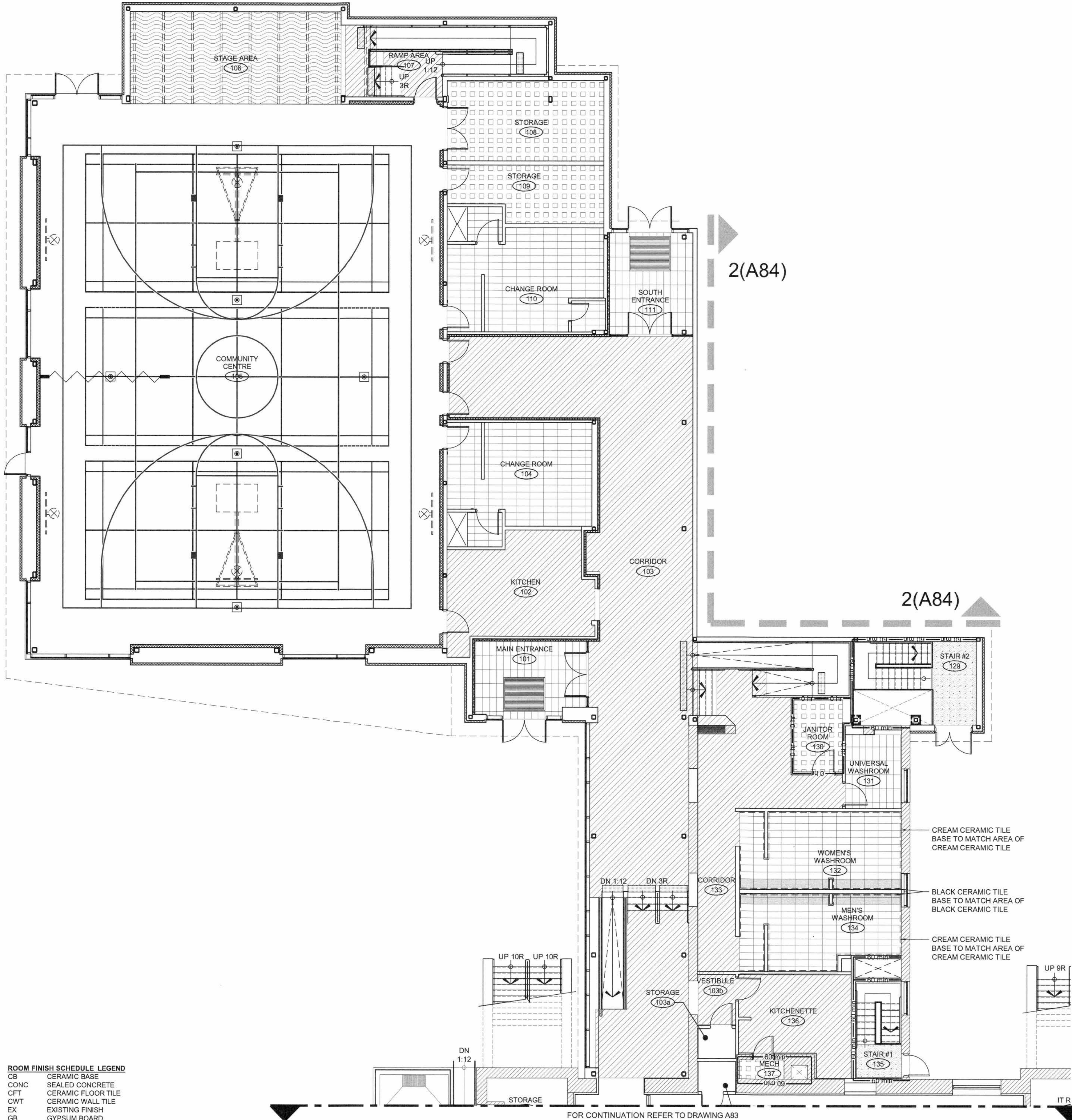
1 PARTIAL GROUND FLOOR - INTERIOR FINISHES SCALE: 1/8\"/>
