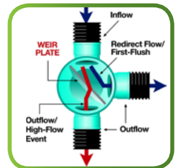
WEIR STRUCTURE
