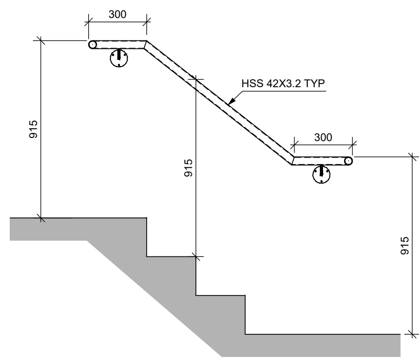
SECTION SCALE - 1:20
