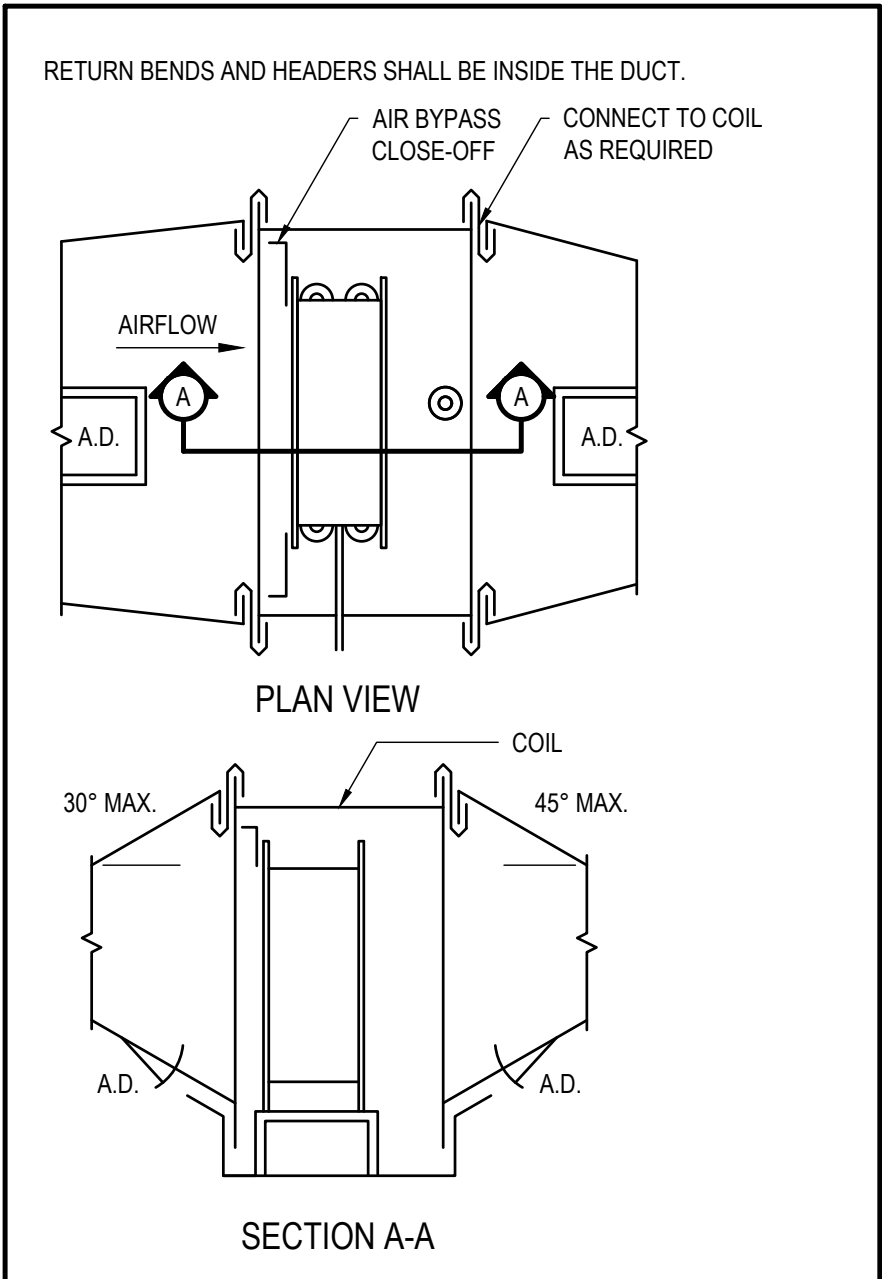
2 M402 TYPICAL HEATING COIL INSTALLATION DETAIL SCALE: N.T.S.
